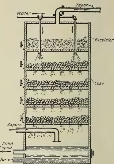
FIG. 62.—Hurdle Scrubber Filled with Coke.
